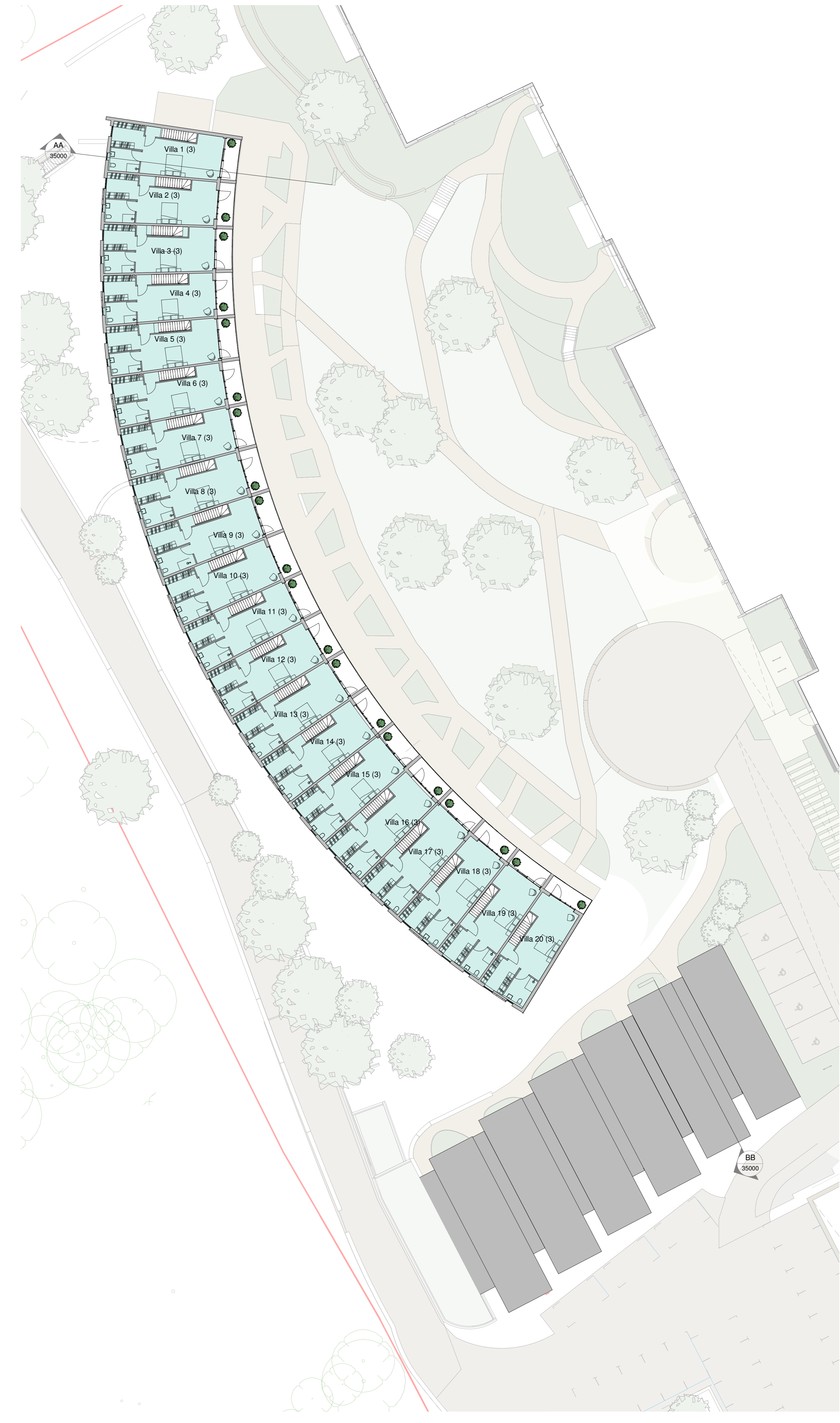
Second Floor - Proposed 1 : 200
